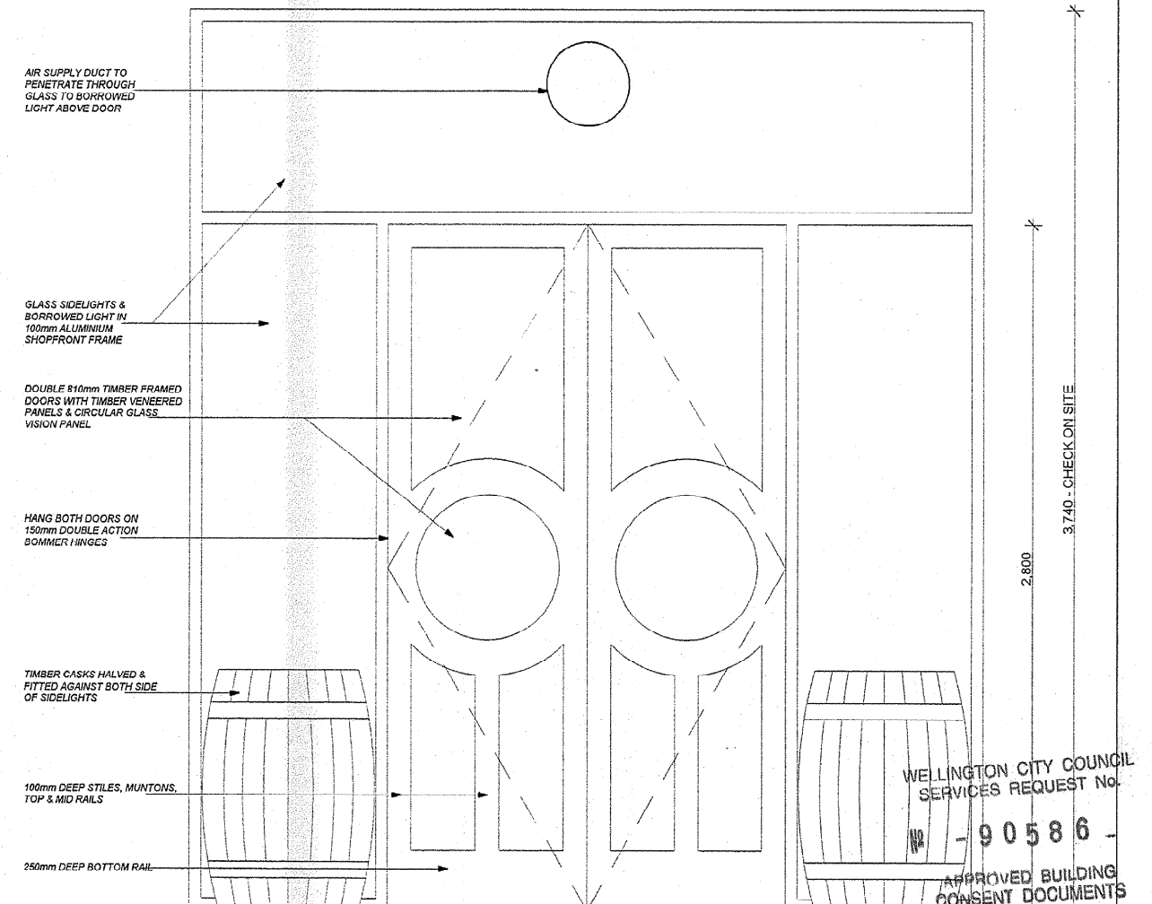
ELEVATION OF DOORS TO SERVERY SCALE 1:20
