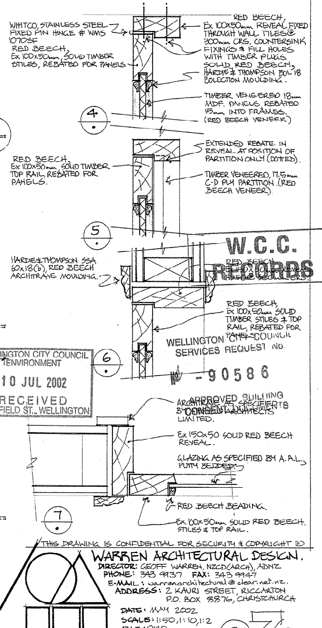
ELEVATION H
