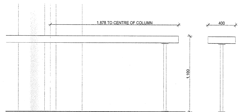
ELEVATION OF LEANER C SCALE 1:20
