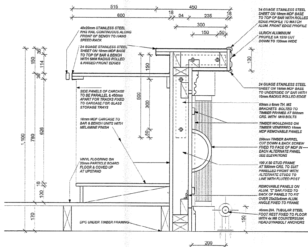
SECTION A THROUGH BAR SCALE 1:10
