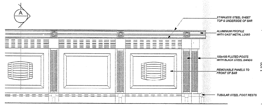
TYPICAL BAR ELEVATION SCALE 1:20
