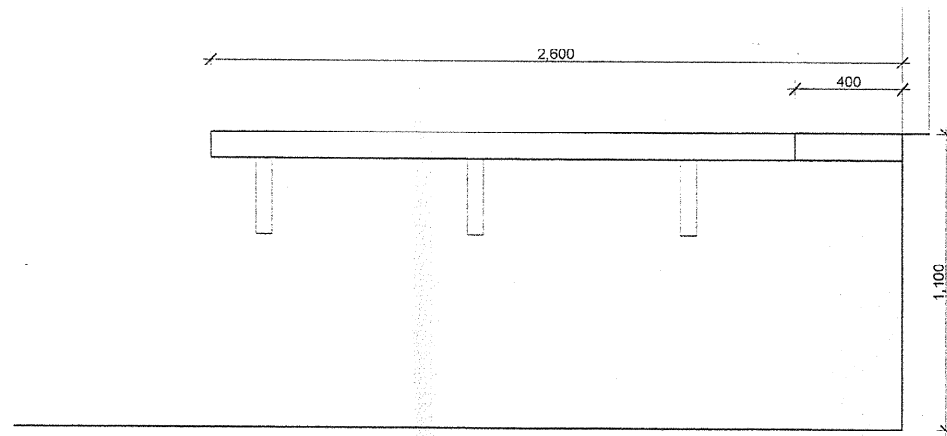
ELEVATION OF LEANER A SCALE 1:20
