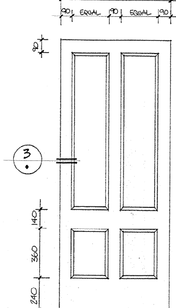
DOORS 1D12, 1D13, 1D14, 1D16
