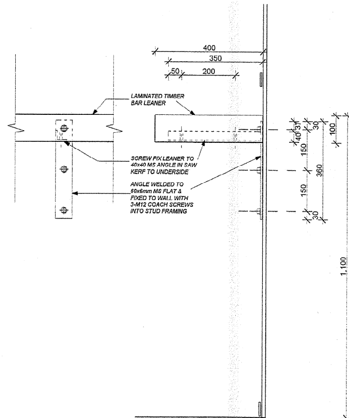
DETAILS FOR LEANER A SCALE 1:10
