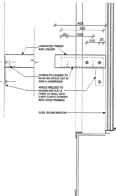
DETAILS FOR LEANER B SCALE 1:10
