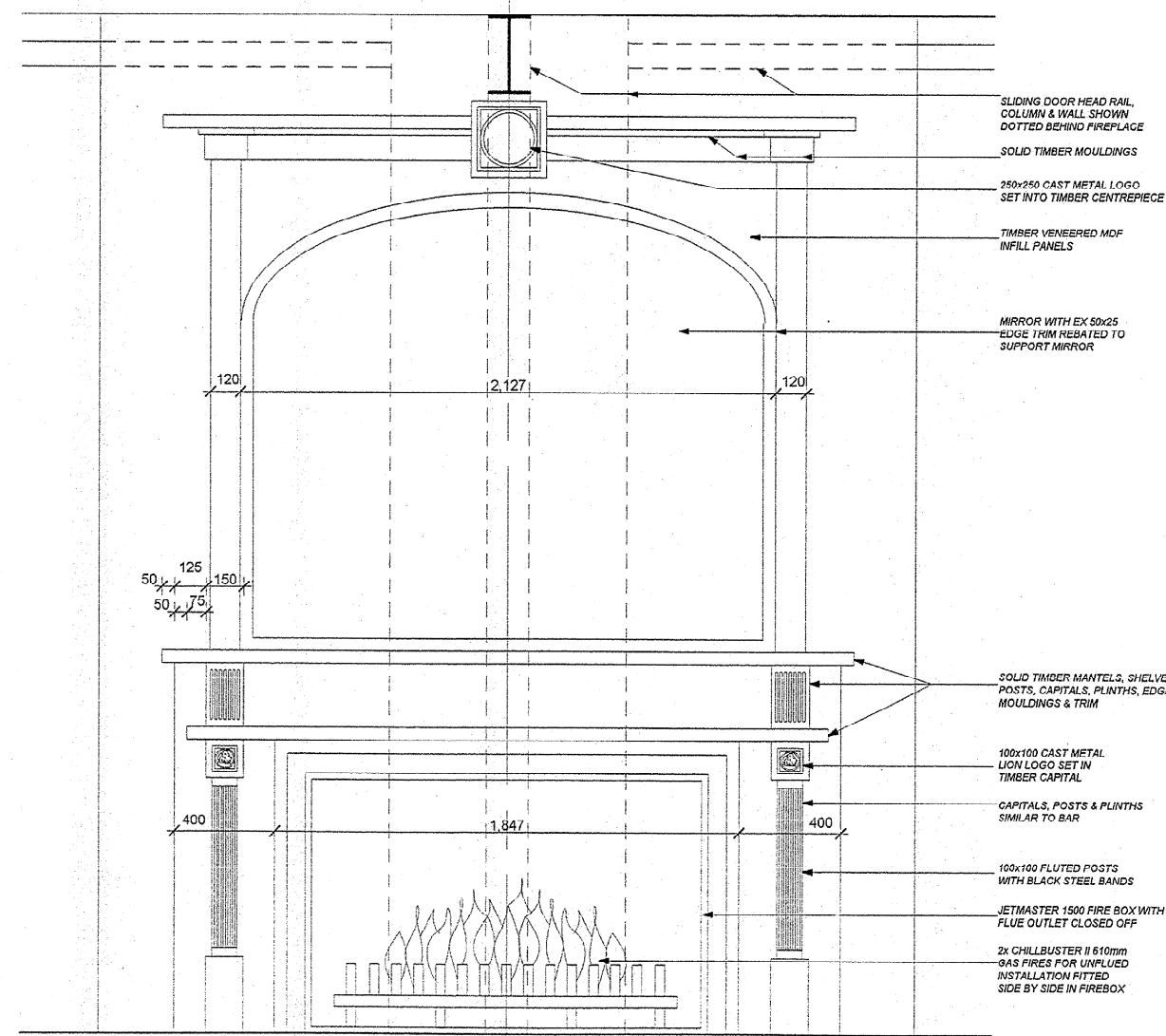
ELEVATION OF FIREPLACE SCALE 1:20
