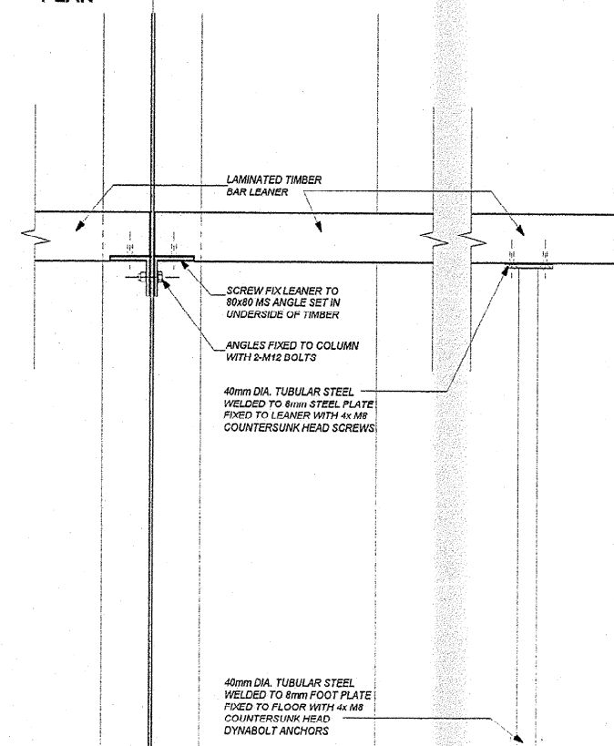
DETAILS FOR LEANER C SCALE 1:10
