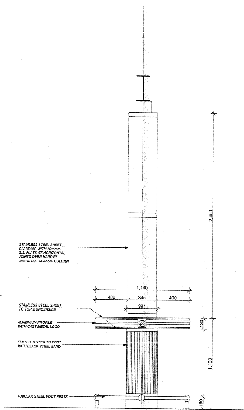
ELEVATION OF LEANER D SCALE 1:20
