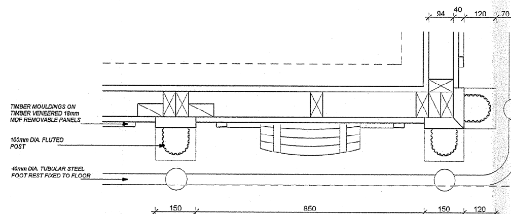
PART PLAN SCALE 1:10
