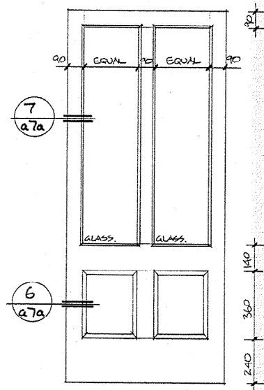
DOORS 1D18, 1D04
