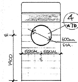
ELEVATION K
