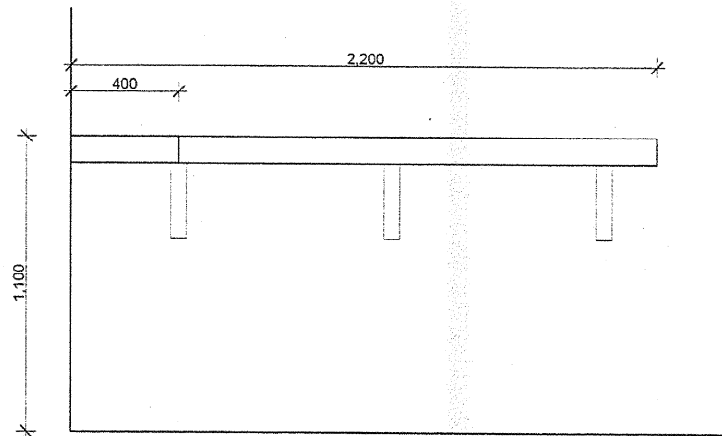
ELEVATION OF LEANER A SCALE 1:20
