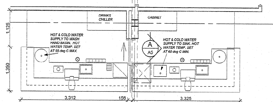
PLAN OF BAR SCALE 1:50
