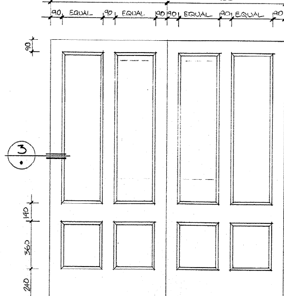
DOORS 1D15
