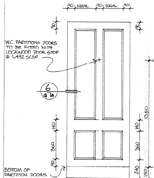
DOORS 1D05, 1D07, 1D08 W.C. PARTITION DOORS x 3
