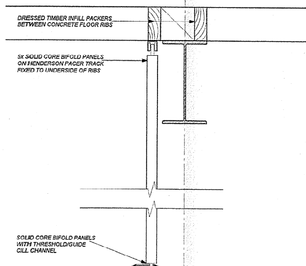
DETAIL AT BIFOLD DOOR
