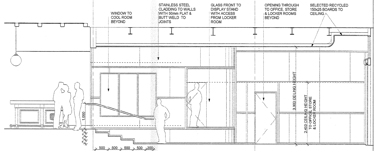
CABLE ST ENTRANCE ELEVATION
