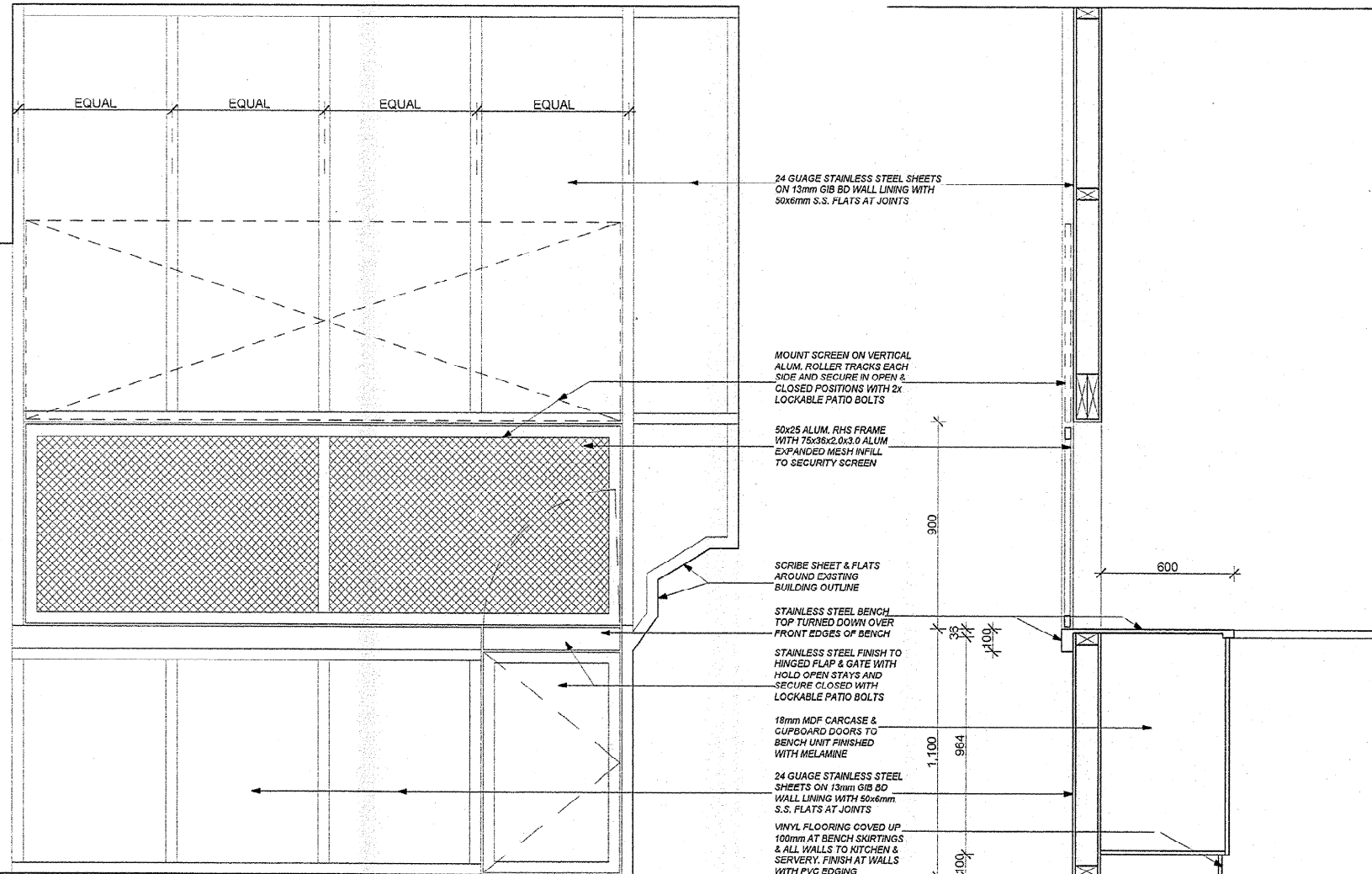
ELEVATION OF OUTDOOR SERVERY SCALE 1:20
