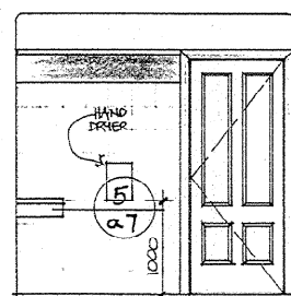
ELEVATION P
