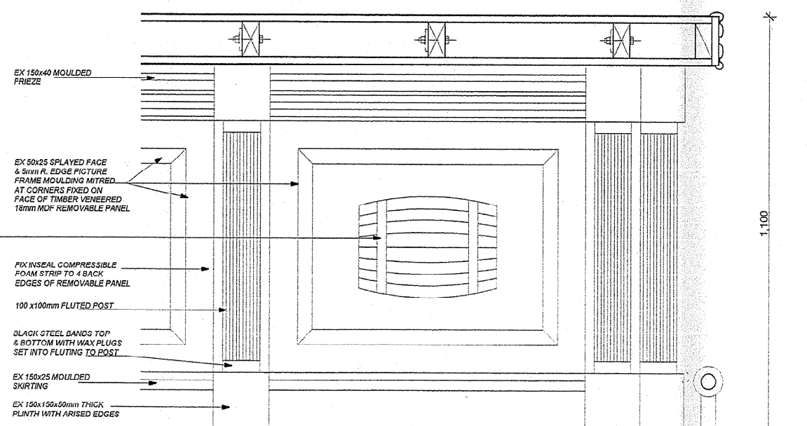
ELEVATION OF BAR FRONT SCALE 1:10
