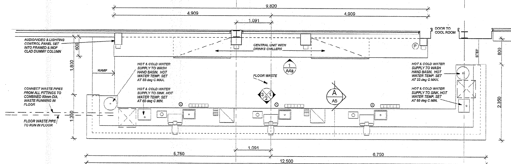
PLAN OF BAR SCALE 1:50 GROUND FLOOR BAR / RESTAURANT
