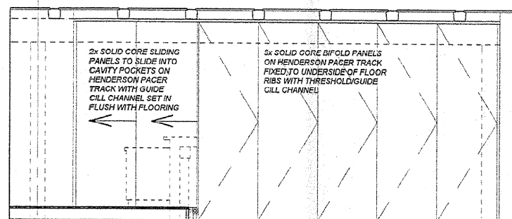
SLIDING / BIFOLD DOOR ELEVATION
