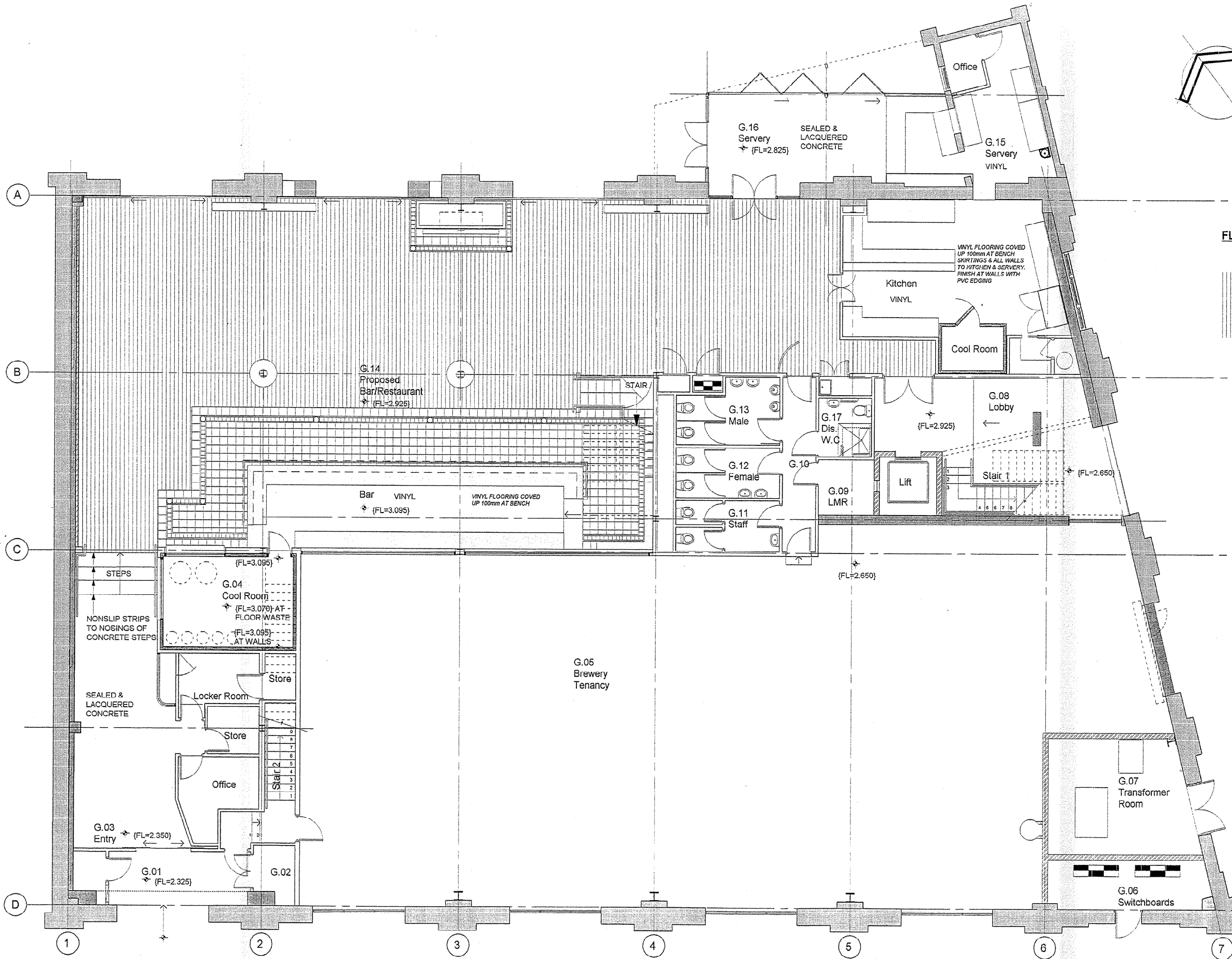
GROUND FLOOR FINISHES SCALE 1:100
