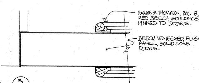
DOORS 1D13 & 1D16 TO BE METAL CLAD ON ONE SIDE, AS PER DETAIL 2 ON THIS PAGE.
