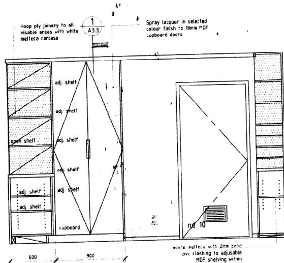
Copier Room Elevation 01 125 A3.3
