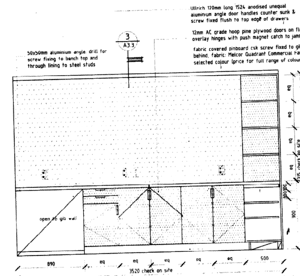
Copier Room Elevation 04 125 A3.3
