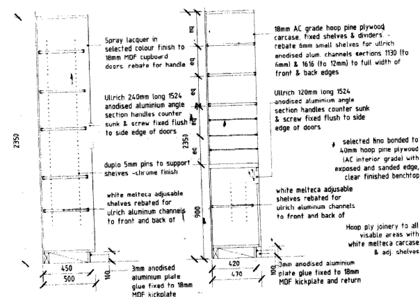
Section 1 125 A3.2
