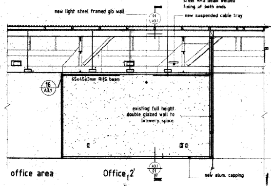
05 Interior Elevation to Office 2 2.2 1:50
