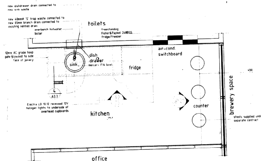
Kitchen Plan 02 125 A3.3
