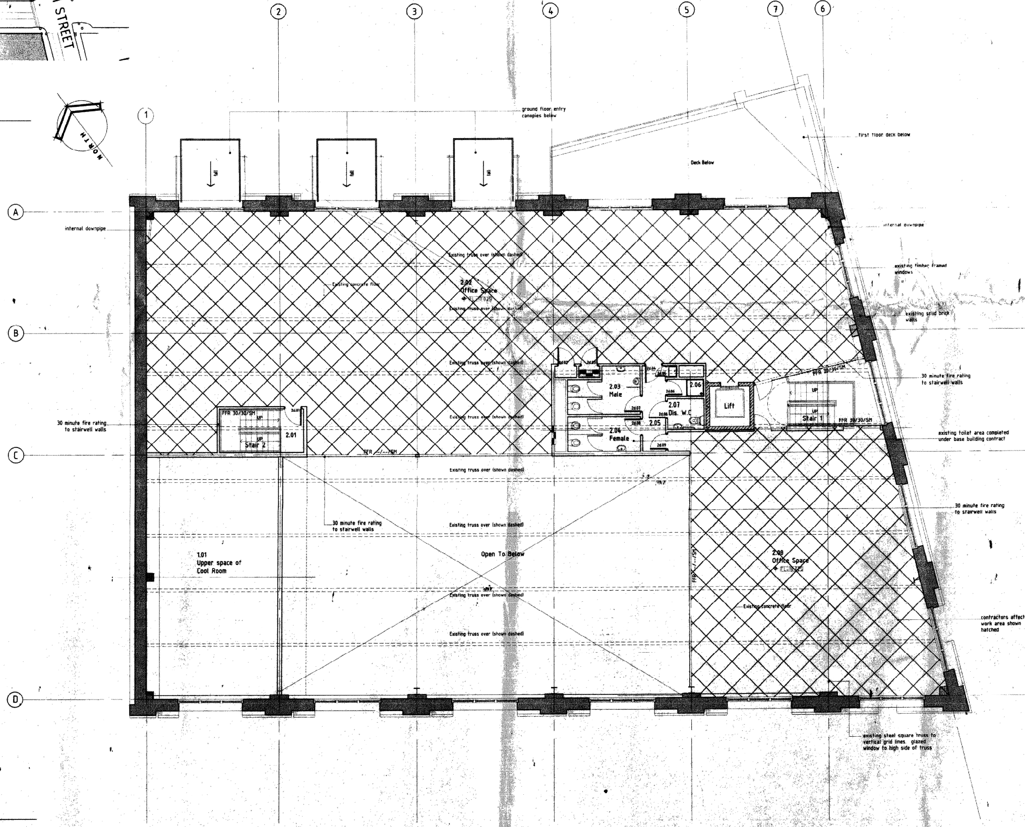
01 Existing Second Floor Plan 1:100
