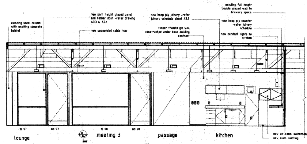
04 Interior Elevation to Main Office Space 2.2 1:50
