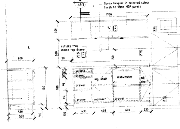
Section 2 125 A3.3
