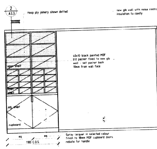
Copier Room Elevation 02 125 A3.3
