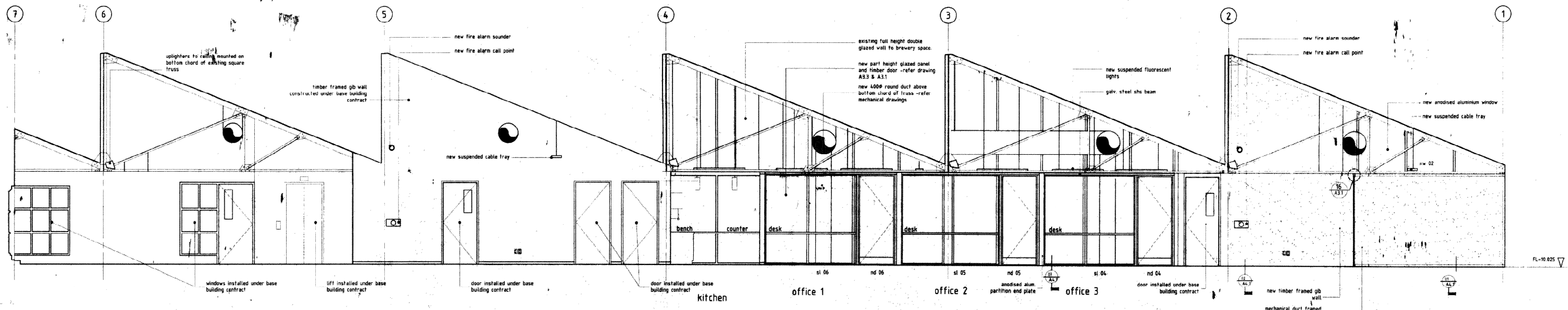
02 Interior Elevation 2.2 1:50
