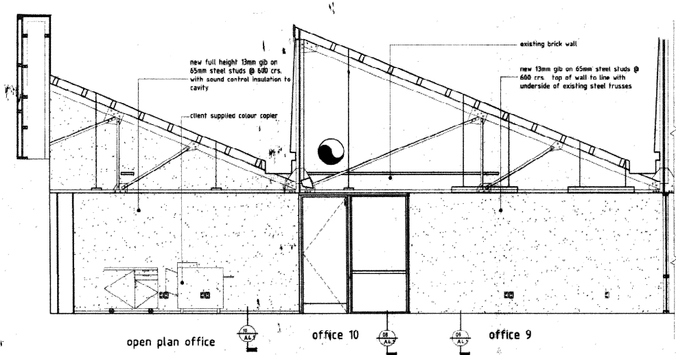
03 Interior Elevation to Office Space 2 2.2 1:50
