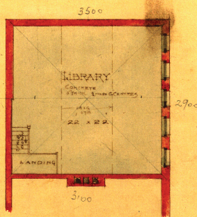
# THIRD FLOOR PLAN # OF LIBRARY #
