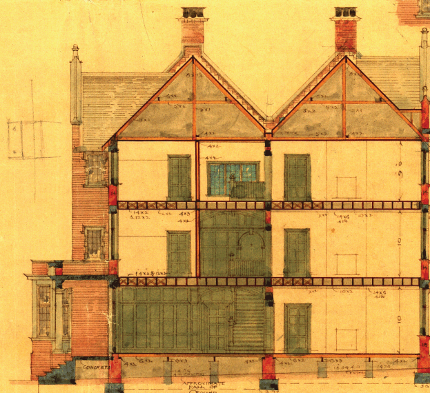
# GROUND SECTION #
